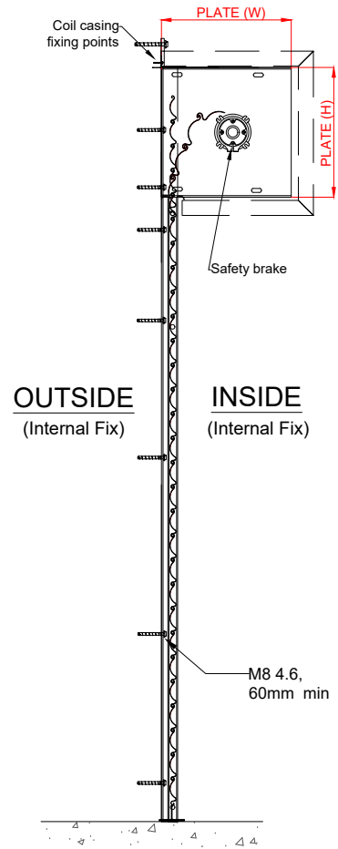
TYPICAL THROUGH SECTION
