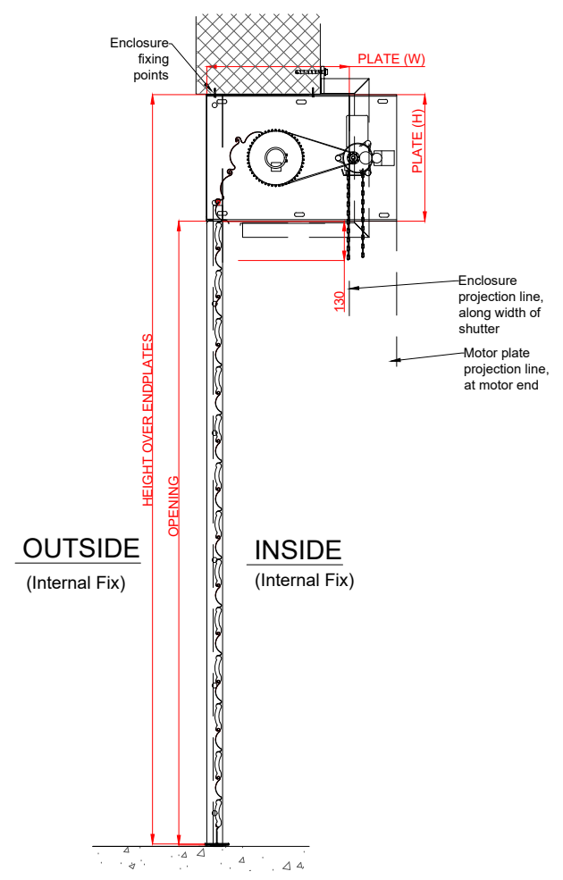
TYPICAL THROUGH SECTION
