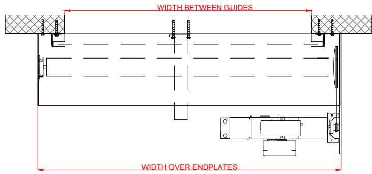
ELEVATION VIEWED FROM INSIDE
