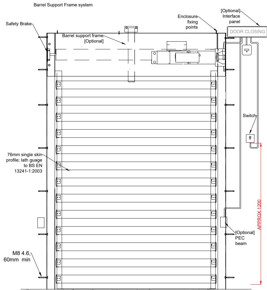
ELEVATION VIEWED FROM INSIDE
