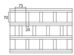
75mm brick bond spacing (surcharge)
