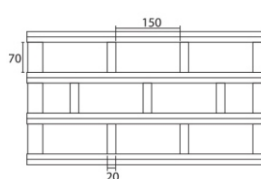
150mm brick bond spacing
