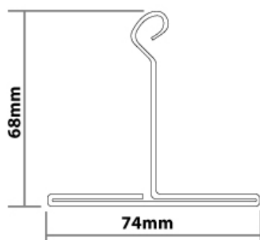
"T" section
