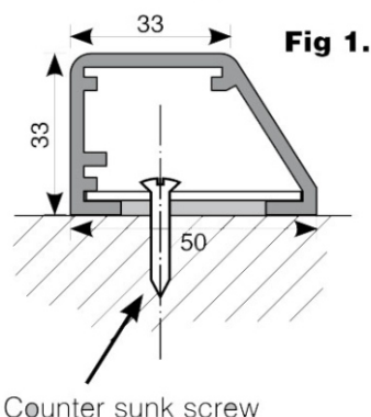
Aluminium guide and fixing plate
