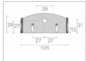
Bracket dimensions
